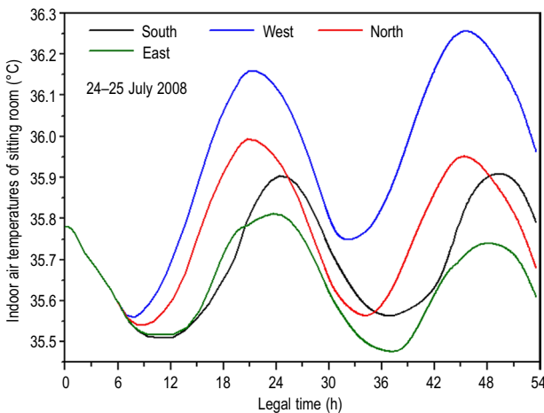
Fig. 9. Sitting room temperatures in the case of massive brick S/V ratio = 0.27, July 24 and 25, 2008
